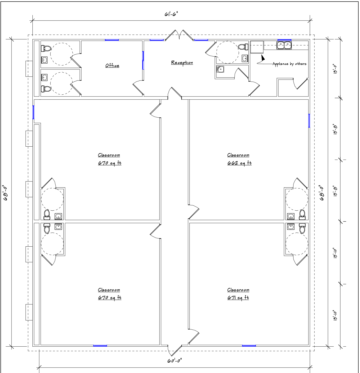
Floor Plan
