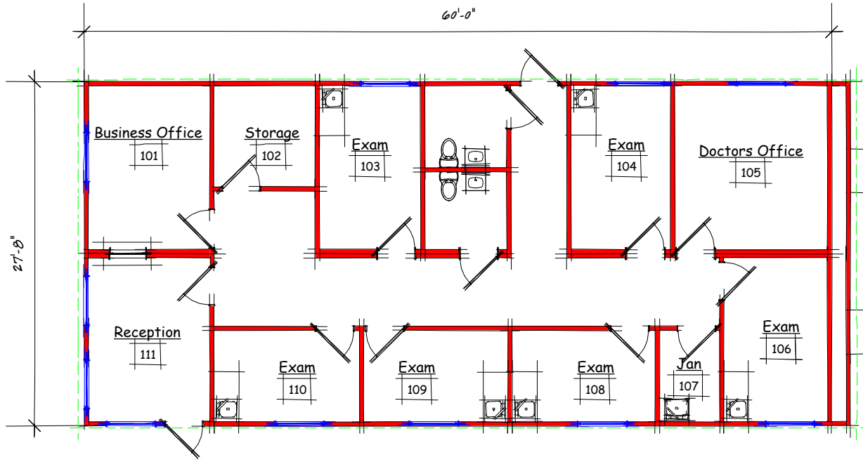
Floor Plan
