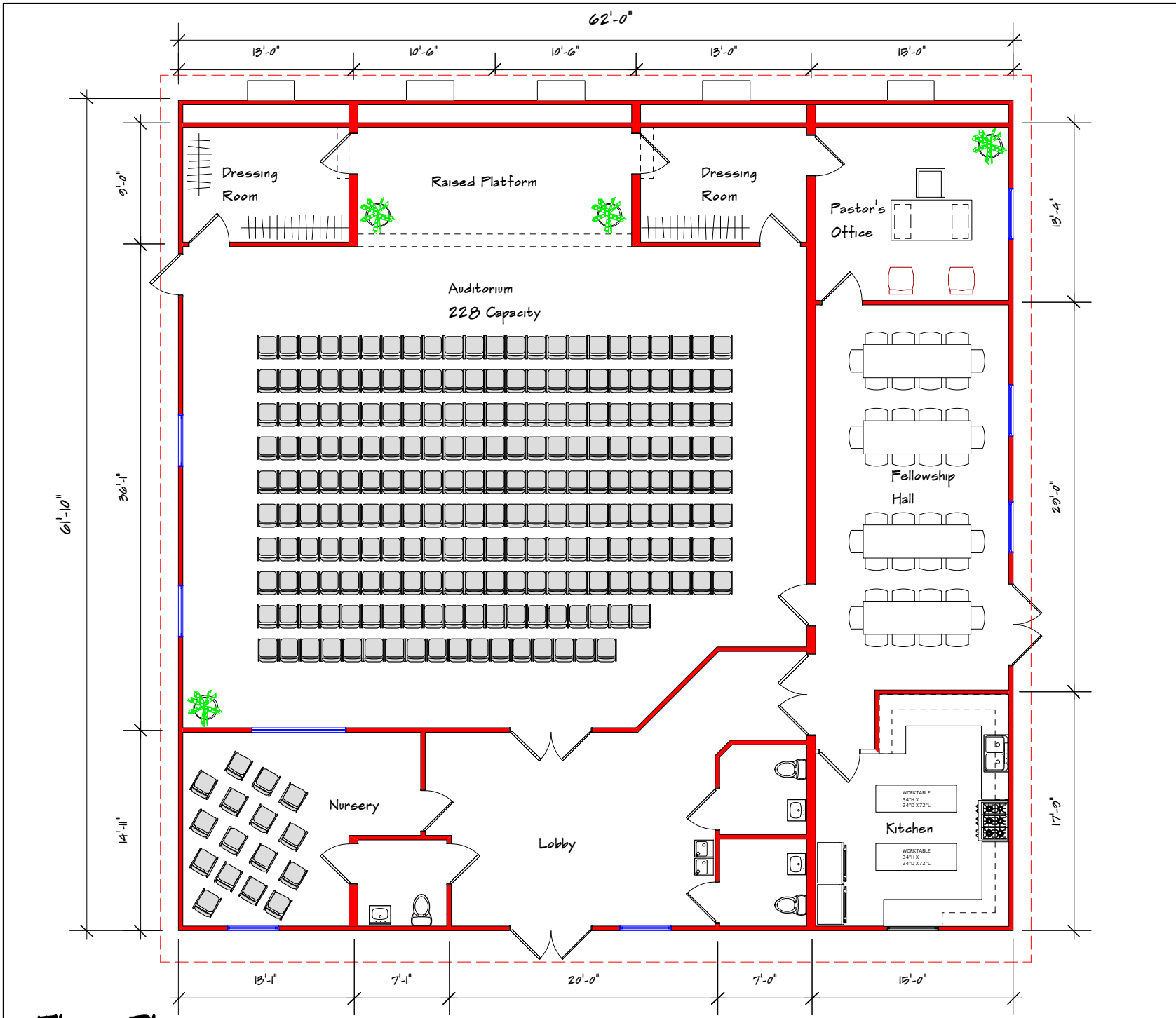
Floor Plan
