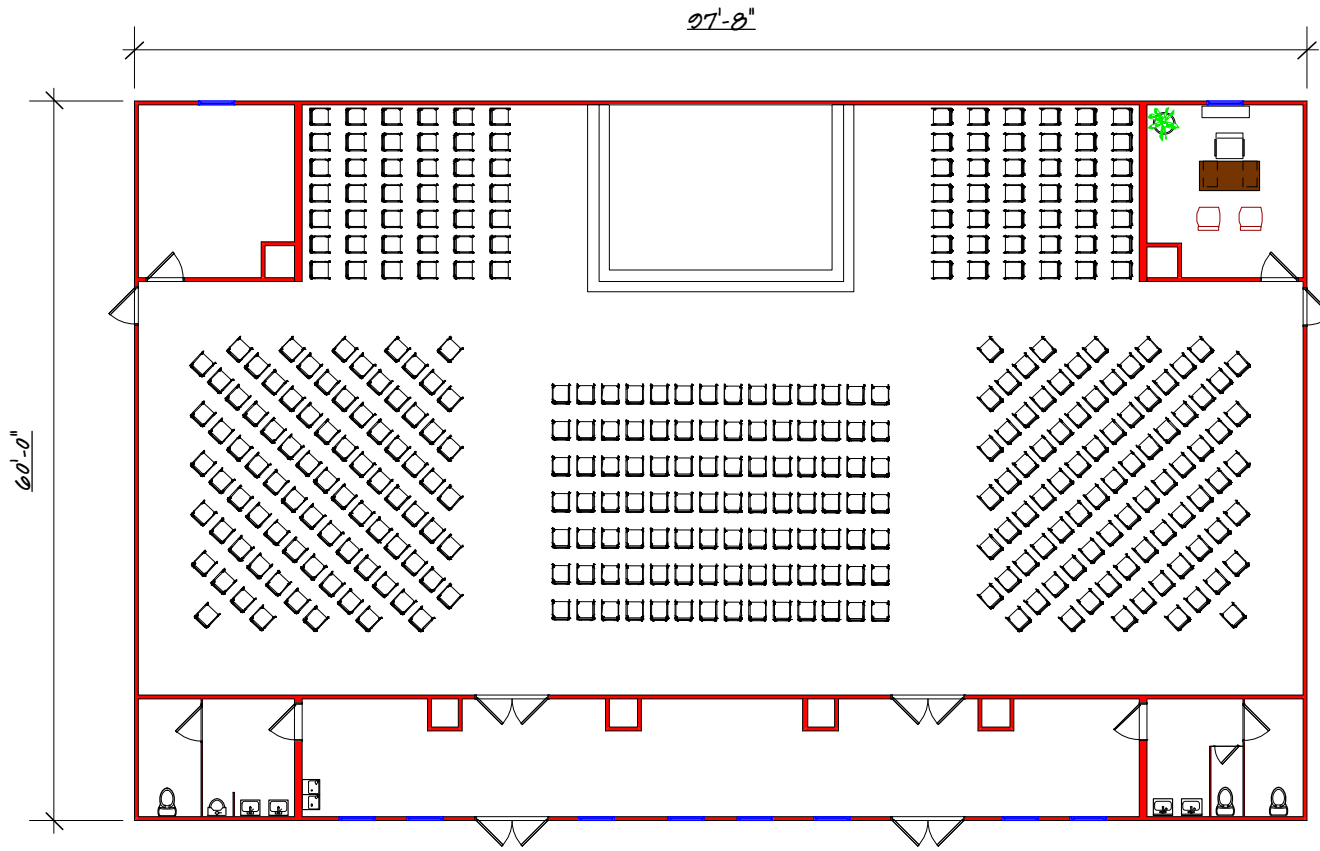
Floor Plan
