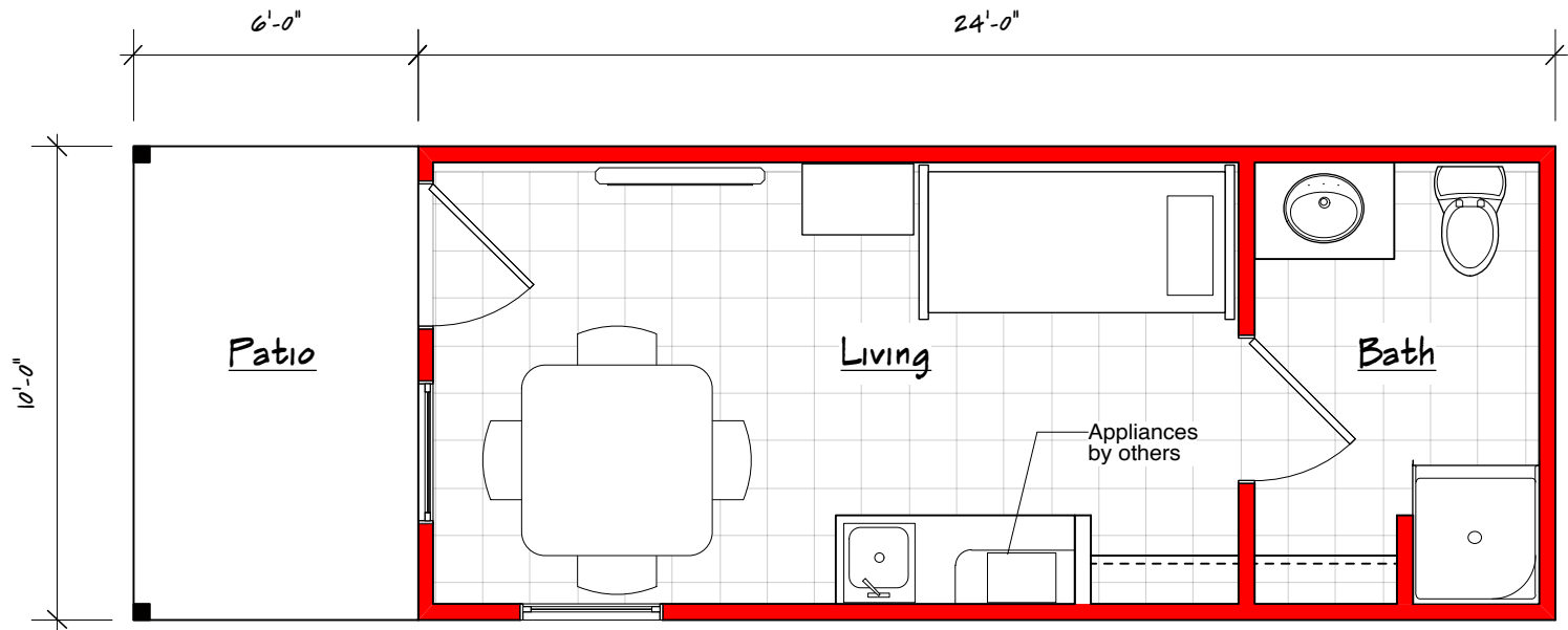
Floor Plan
