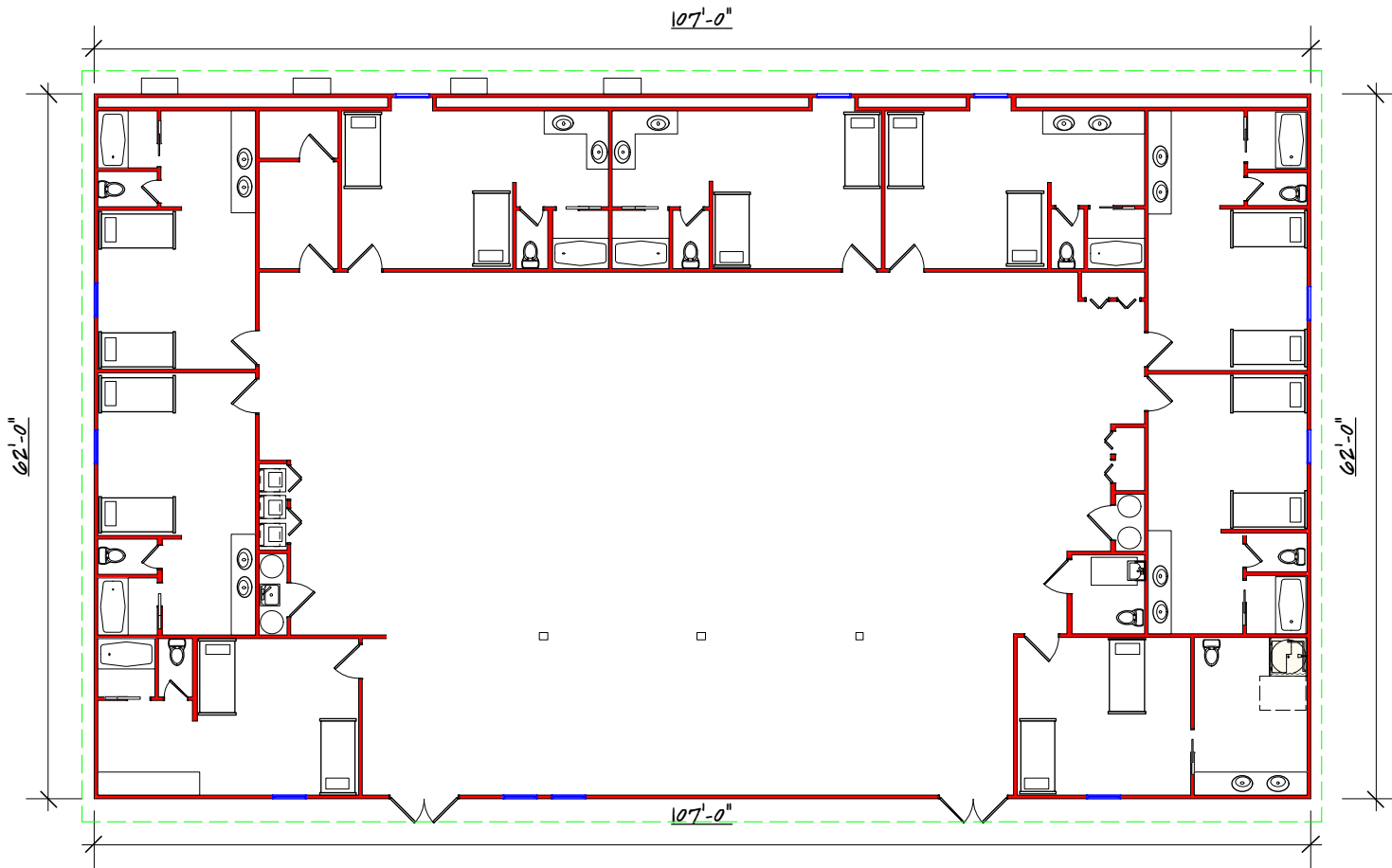
Floor Plan
